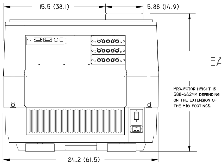
Figure 2-2 Model 250, rear view showing height and width (in mm).
