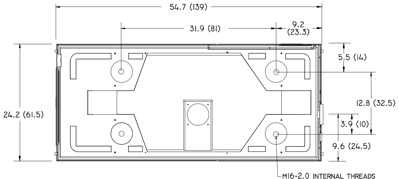
Figure 2-1 Model 250 Projector, footprint.
