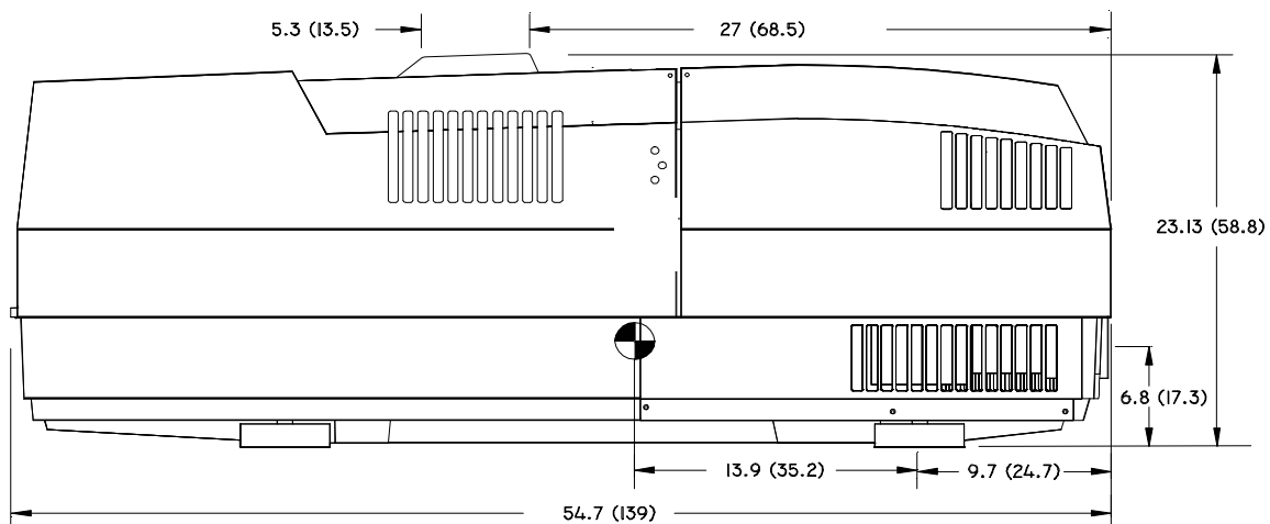
Figure 2-3 Model 250 Right Side View. The 173mm distance from center of lens to bottom of foot is with foot set to minimum extension.
