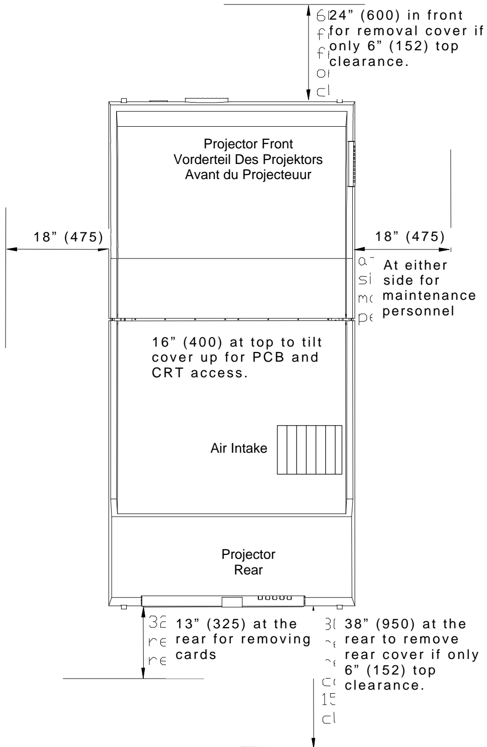
Figure 2-4 Clearances in inches (mm) for cover removal and physical access.
